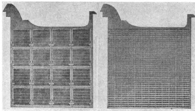
A Comparison of Ordinary Positive and Negative Grids.
